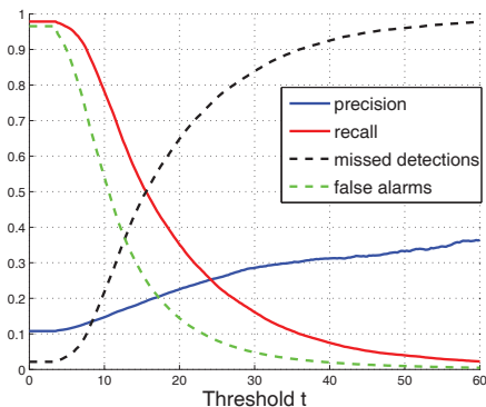
Fig. 3. Precision, recall, missed detection probability and false alarm probability (using real VAD output) for overlap detection
