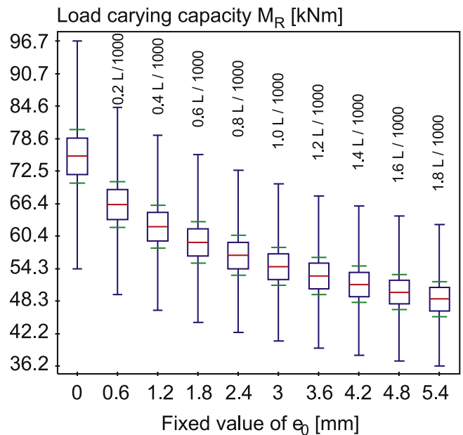
Fig. 10 – Box-whisker plots for \bar{\lambda}_{LT} = 0.93 .
