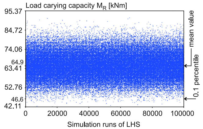
Fig. 4 – Statistical analysis M_R for \bar{\lambda}_{LT} = 0.9 ( L = 2.85 m).
