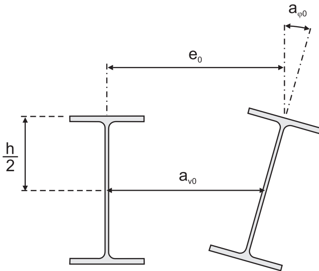
Fig. 3 – Amplitudes of initial deflections e_0 , a_{v_0} and rotation a_{\varphi_0} .
