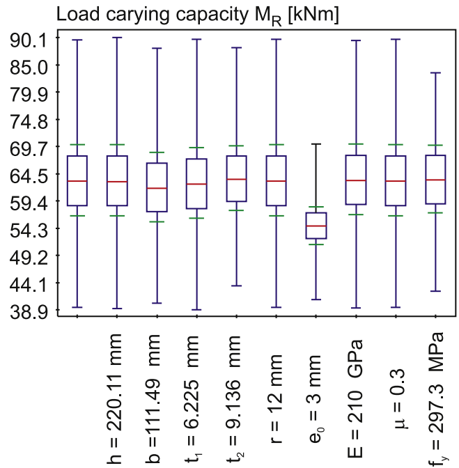
Fig. 9 – Box-whisker plots for \bar{\lambda}_{LT} = 0.93 .
