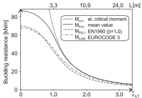
Fig. 13 – Statistical analysis of inelastic buckling resistance M_P .
