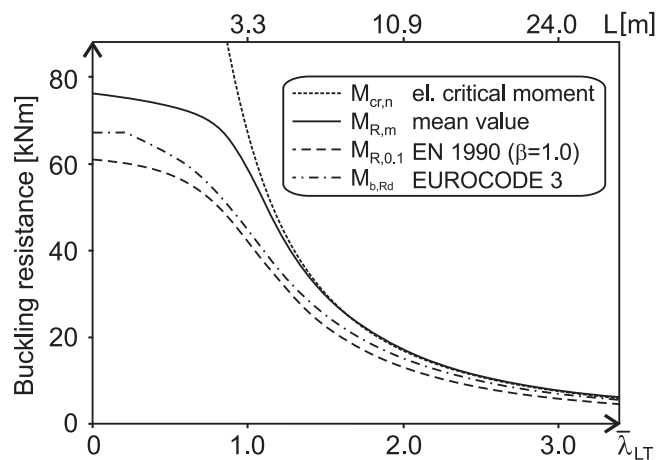
Fig. 5 – Statistical analysis of M_R .
