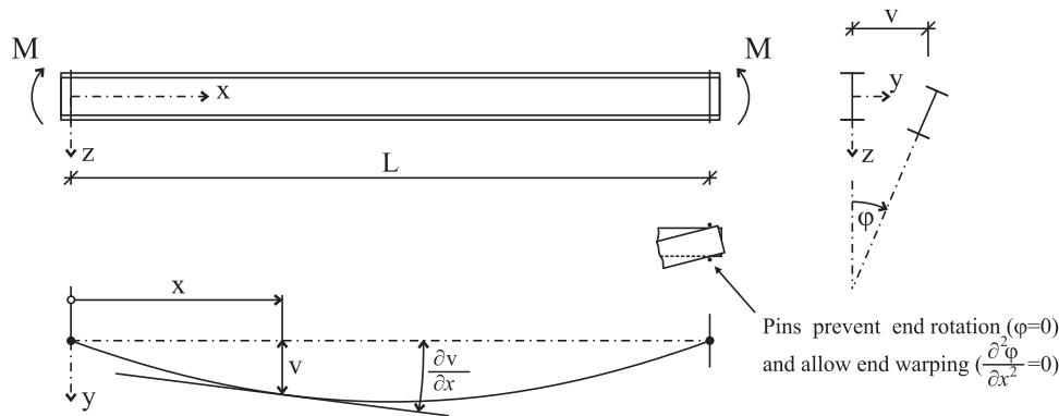
Fig. 2 – Buckling of simply supported IPE-beam.
