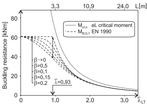
Fig. 12 – Statistical analysis of M_R for varying values of \beta .
