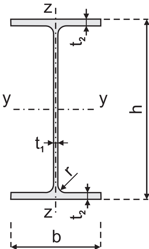
Fig. 1 – IPE cross-section.
