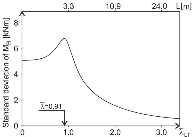
Fig. 6 – Standard deviation of M_R vs \bar{\lambda}_{LT} .
