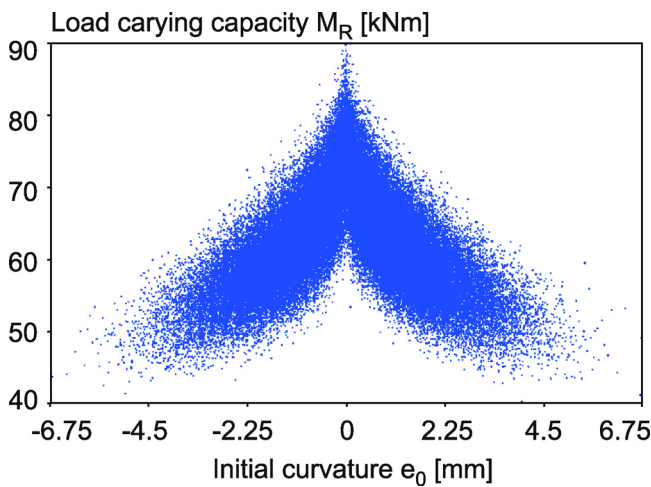
Fig. 8 – Random dependence between e_0 and M_R for \bar{\lambda} = 0.93 .
