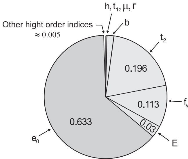
Fig. 7 – Sobol's SA for \bar{\lambda}_{LT} = 0.93 .
