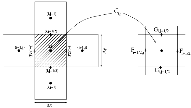
Fig. 1. An illustration of control volumes C_{i,j} used in the proposed method.
