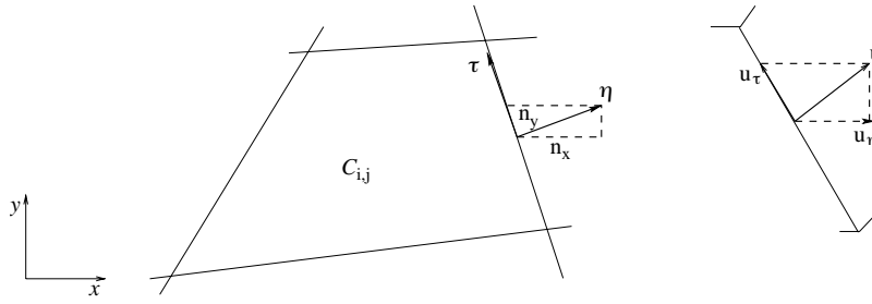
Fig. 2. Illustration of the projected velocities on the control volume C_{i,j} .
