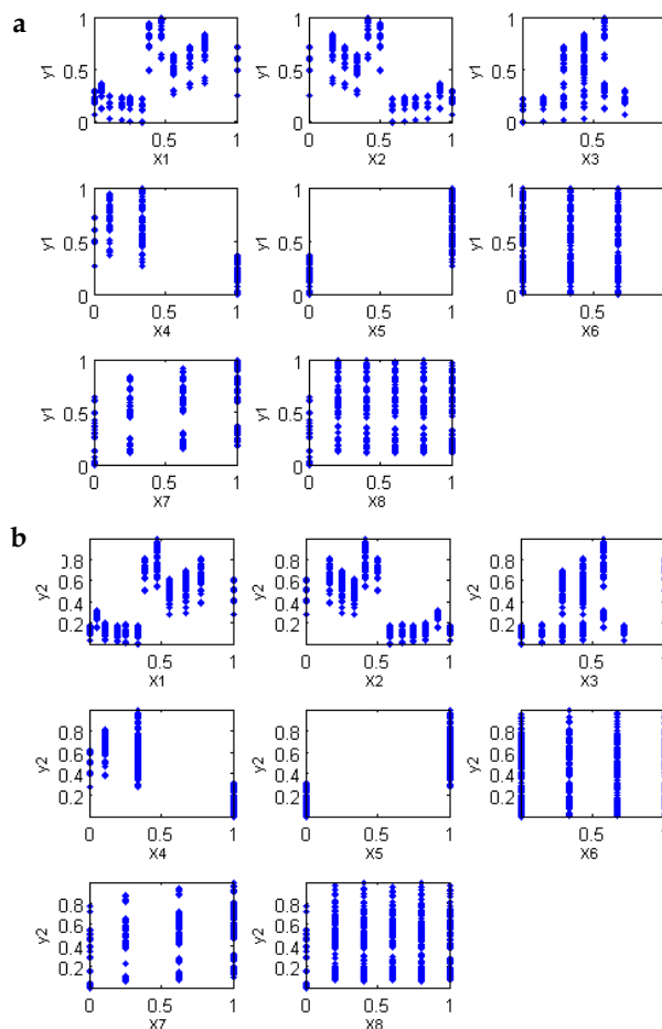
Fig. 2. Scatter plot demonstrating visually the relationship between each normalized input variable and the normalized outputs a) the heating load, or b) the cooling load.
