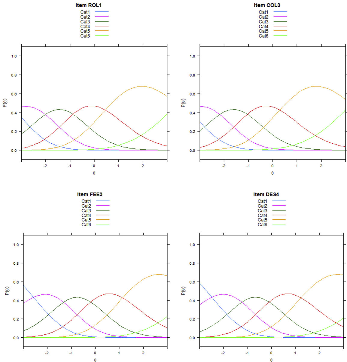
Fig. 3. Category probability curves for selected items. Note. Cat = Response category.
