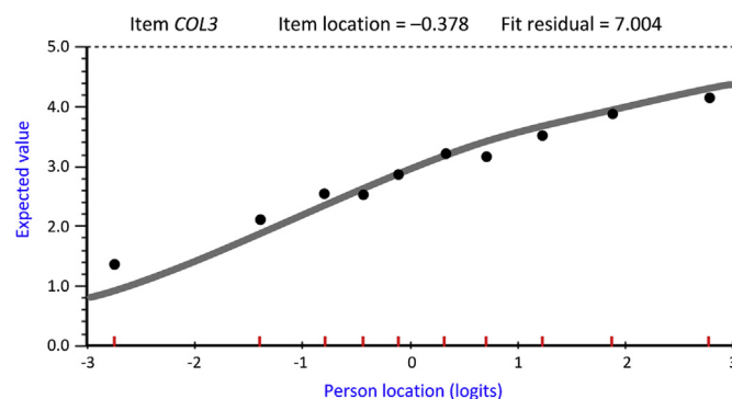
Fig. 2. Item characteristic curve for Item COL3 (during my pre-service training, students helped each other to use ICT in an educational context).
