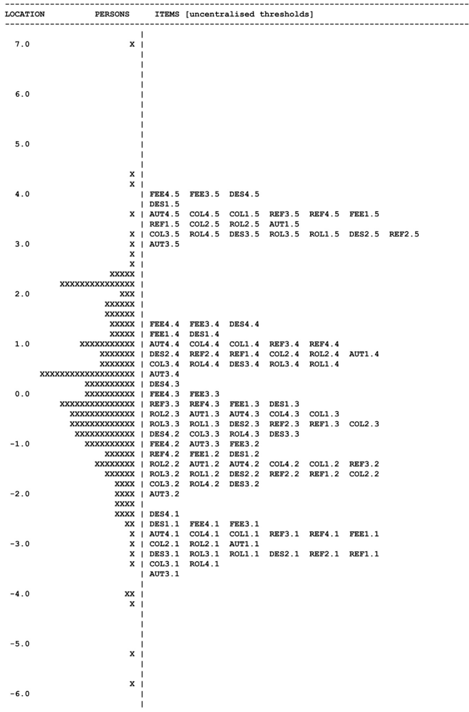
Fig. 4. Person-item (Wright) map of the 22-item SQD-scale. Note. 'X' represents three persons. The Wright map shows the locations of item thresholds (as indicated by "0.1", "0.2", "0.3", "0.4", and "0.5") and person parameters on the logit scale.
