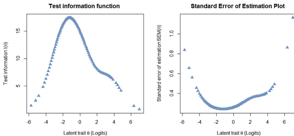
Fig. 5. Test information function and standard error of estimation plot of the 22-item SQD-scale.
