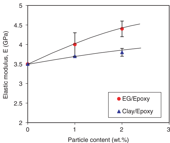
Figure 12. Variation of elastic modulus as a function of particle content. (Reproduced from [50] with permission. © Elsevier 2006.)
