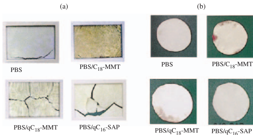
Figure 11. Biodegradability of neat PBS and various nanocomposites sheets: (a) under compost and (b) under soil field. (Reproduced [144], © 2006 John Wiley & Sons, Inc.)
